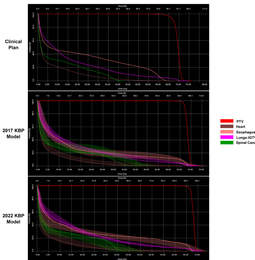
Figure 2 The clinical plan (top), 2017 KBP model plan (middle), and 2022 KBP model plan (bottom) DVHs from a single example case used for model validation. Note that the shaded areas around the KBP model DVHs represent the possible DVH range predicted by the KBP model. Abbreviations: DVH = dose–volume histograms; GTV = gross tumor volume; HQC = high-quality clinical; KBP = knowledge-based planning; PTV = planning target volume.
