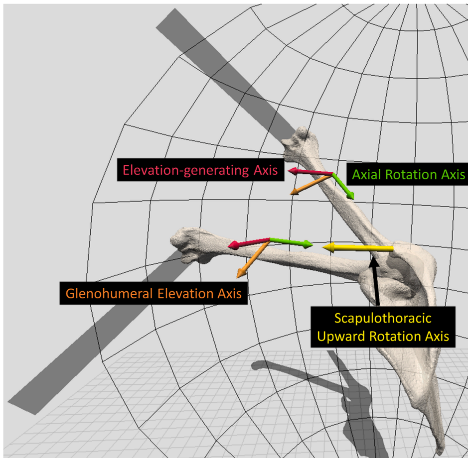
Fig. 3. Illustration of the elevation-generating (red) and axial rotation (green) axes for projection of angular velocity. The axial rotation axis is coincident with the longitudinal axis of the humerus. However, the elevation-generating axis is not coincident with any anatomical axis. It always lies on the transverse plane and an infinitesimal rotation about it causes the humerus to elevate along the superoinferior axis. In contrast, the glenohumeral elevation axis of rotation (orange) does not strictly cause the humerus to elevate along the superoinferior axis because of scapular tilt ( \sim 30^\circ in this illustration). Furthermore, the scapulothoracic upward rotation axis (Euler-based, yellow) and the glenohumeral elevation axis are not co-aligned. Therefore, traditional SHR compares angles of rotation about two different axes of rotation. In contrast, coordinated SHR compares the relative rotations of the glenohumeral and scapulothoracic joints about the same elevation-generating axis. The illustration shows two different orientations of the humerus (but just one for the scapula for visual clarity) to emphasize that all axes of rotation depend on the orientation of the humerus and scapula. (For interpretation of the references to colour in this figure legend, the reader is referred to the web version of this article.)
