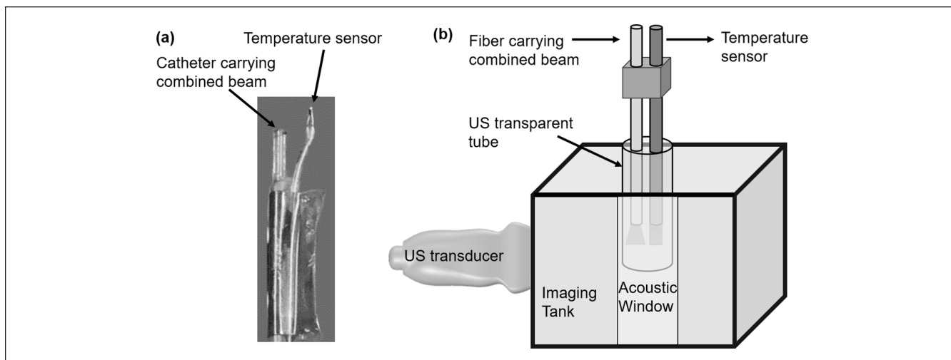
Figure 3. (a) Photograph of the distance between k-type thermocouple and the ablation catheter. (b) Schematic diagram of the experimental setup for evaluating the accuracy of PA thermometry. The power rating of the CW laser beam was varied from 0 W (OFF state) and 4, 8, 10 W. PA images were acquired at 500 FPS.
