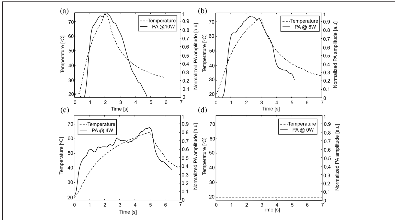
Figure 5. Fast PA imaging for monitoring rapid temperature changes induced by laser ablation. (a-d) portrays the measurements of temperature with fast (500 Hz) PA imaging followed the k-type thermocouple readings. The solid lines indicate the normalized PA amplitude due to temperature variations (indicated by dashed lines) caused by a CW laser at different power ratings.
